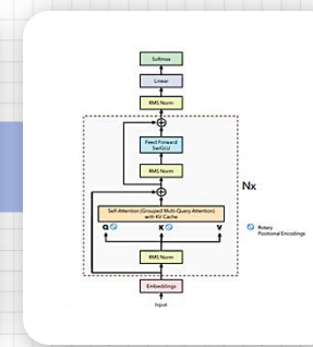
Transformer时代 (Attention)
